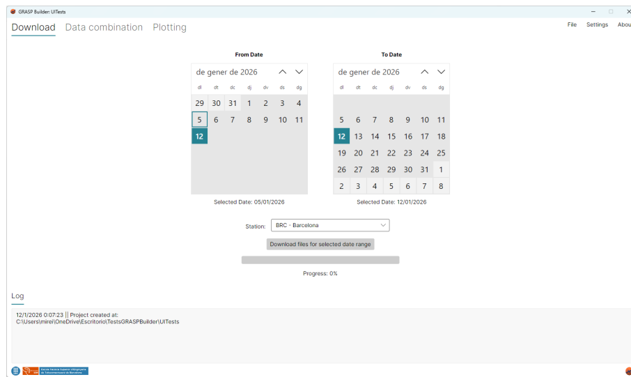
Figure 24: Download view
