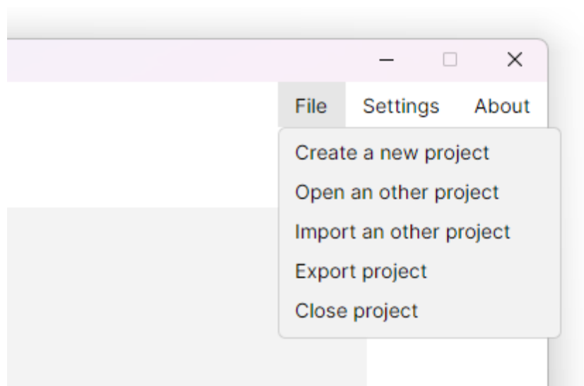
Figure 10: Menu options
