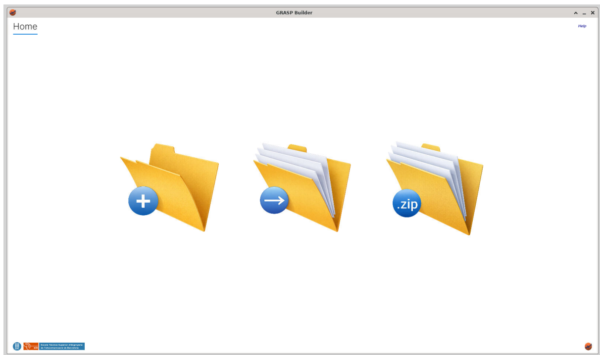
Figure 28: Home screen
