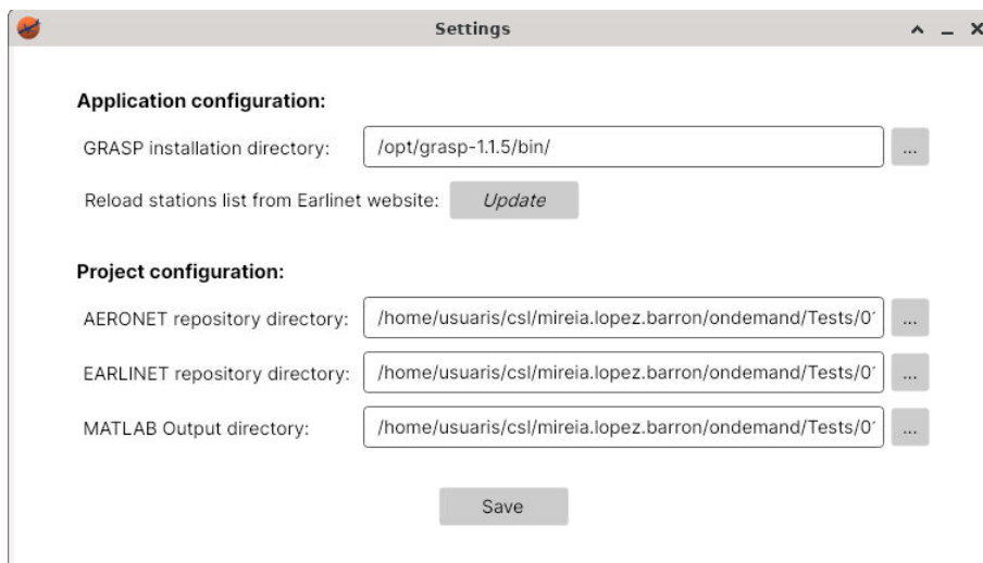
Figure 27: Settings window
