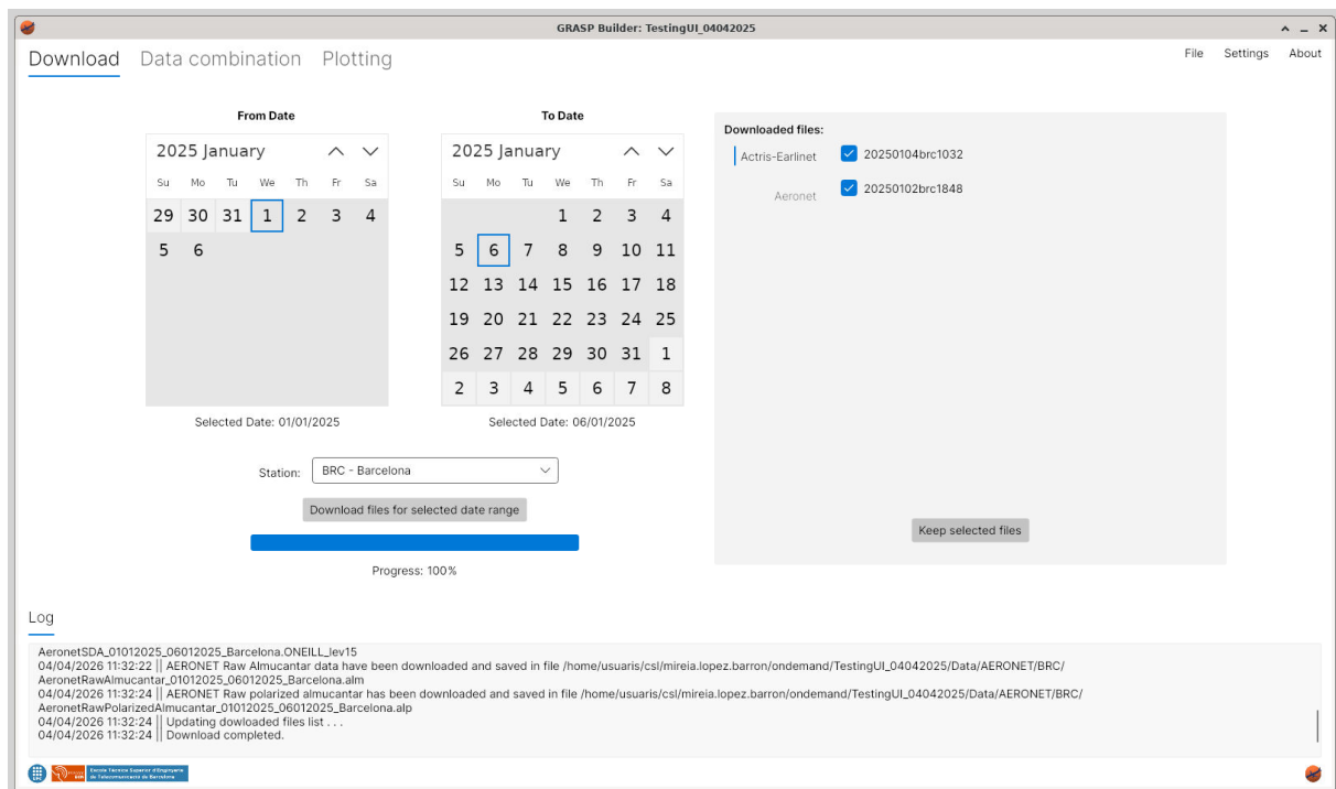
Figure 29: Files downloaded
