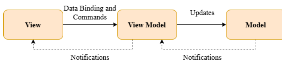
Figure 17: MVVM design pattern
